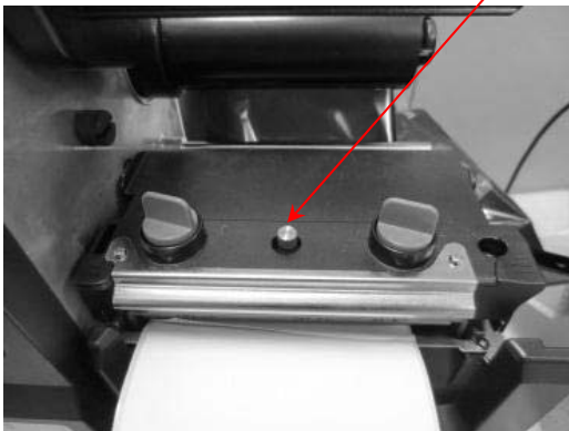
Printhead Thumbscrew
