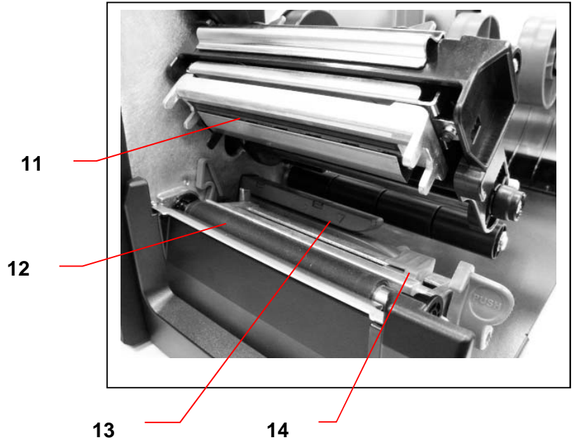
Figure 3. Printer Interior View
